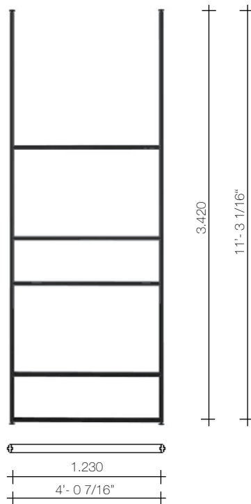
Vertical studs and cross profiles
